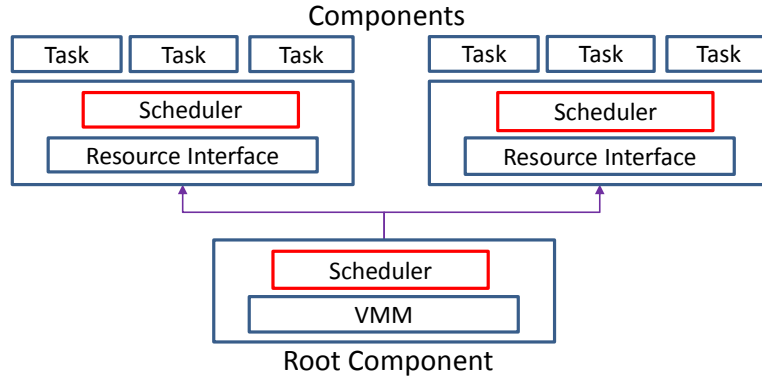
Figure 2.2: Compositional Scheduling Architecture
