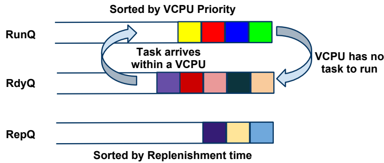
Figure 2.3: Scheduler Queues in RT-Xen 1.0
